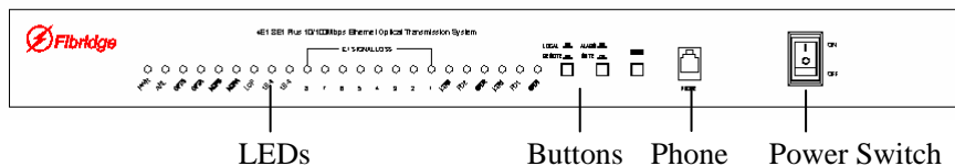
Figure3 Front Panel of the 4/8E1 Multiplexer standalone
